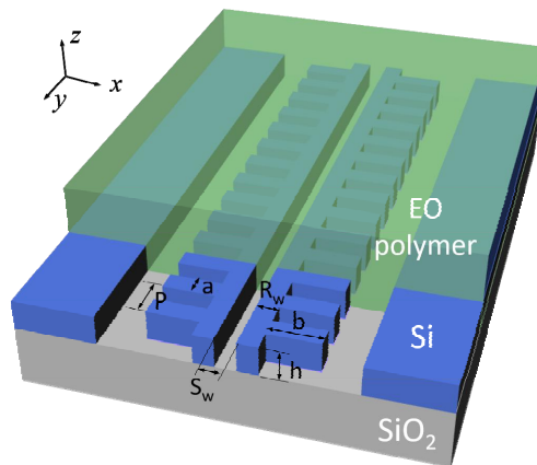
Figure 1. Schematic of the proposed 1D PC slot waveguide filled with EO polymer as a phase shifter for EO modulators.
