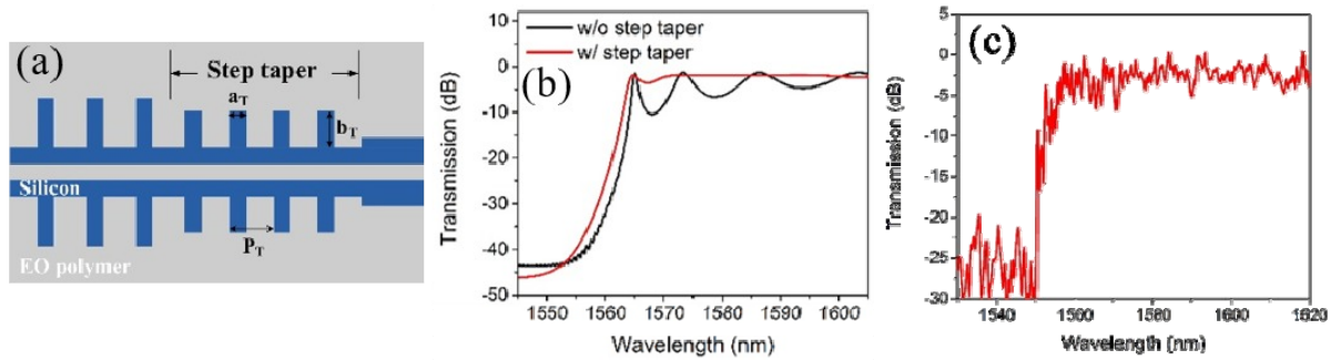
Figure 3. (a) Schematic of the step taper; (b) Simulated transmission spectrum comparing 1D PC slot waveguide with (red curve) and without step taper (black curve); (c) Measured transmission spectrum of 1D PC slot waveguide with optimized step taper.
