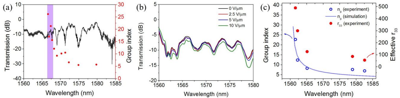
Figure 5. (a) Measured transmission spectrum of the MZI structure and derived group index as a function of wavelength; (b) Measured transmission spectra of the MZI modulator with different DC electric field applied on the electrodes; (c) Group index (from both simulation and experiment) and effective r_{33} as a function of wavelength.
