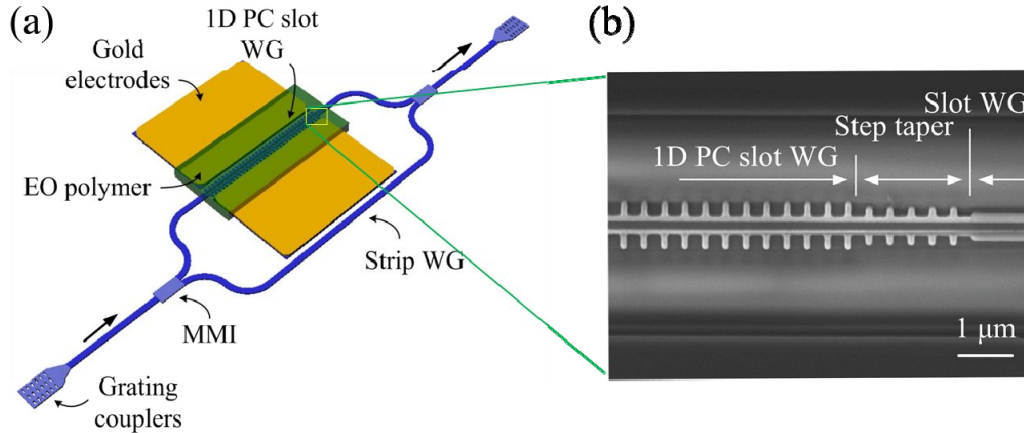
Figure 4. (a) Schematic of a MZI modulator based on 1D PC slot waveguide; (b) scanning electron microscope (SEM) images of the 1D PC slot waveguide and step taper.
