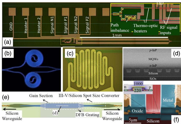
Fig. 4. Active devices on an SOI platform. (a) Optical microscope image of the asymmetric MZI modulator. Inset: magnified detail of the 50/50 Y-junction, optical path imbalance, thermo-optic heaters, and RF signal inputs [37]. (b) Optical microscope images of a spiral-arm asymmetric MZI [36]. (c) Aluminum heater sits on top of one arm of the spiral MZI [36]. (d) SEM image of the longitudinal cross section of the gain region shown in Fig. 4(e) [69]. (e) Schematic of the III-V-on-silicon DFB laser [69]. (f) Cross section view of the photodetector shown in false color to distinguish the materials. Inset shows schematic of the silicon waveguide with dimensions labeled in nanometers, and with TE mode at 2 \mu\text{m} overlaid [38]. Figures are reproduced from: (a) Ref. [37]; (b) and (c) Ref. [36]; (d) and (e) Ref. [69]; (f) Ref. [38].
